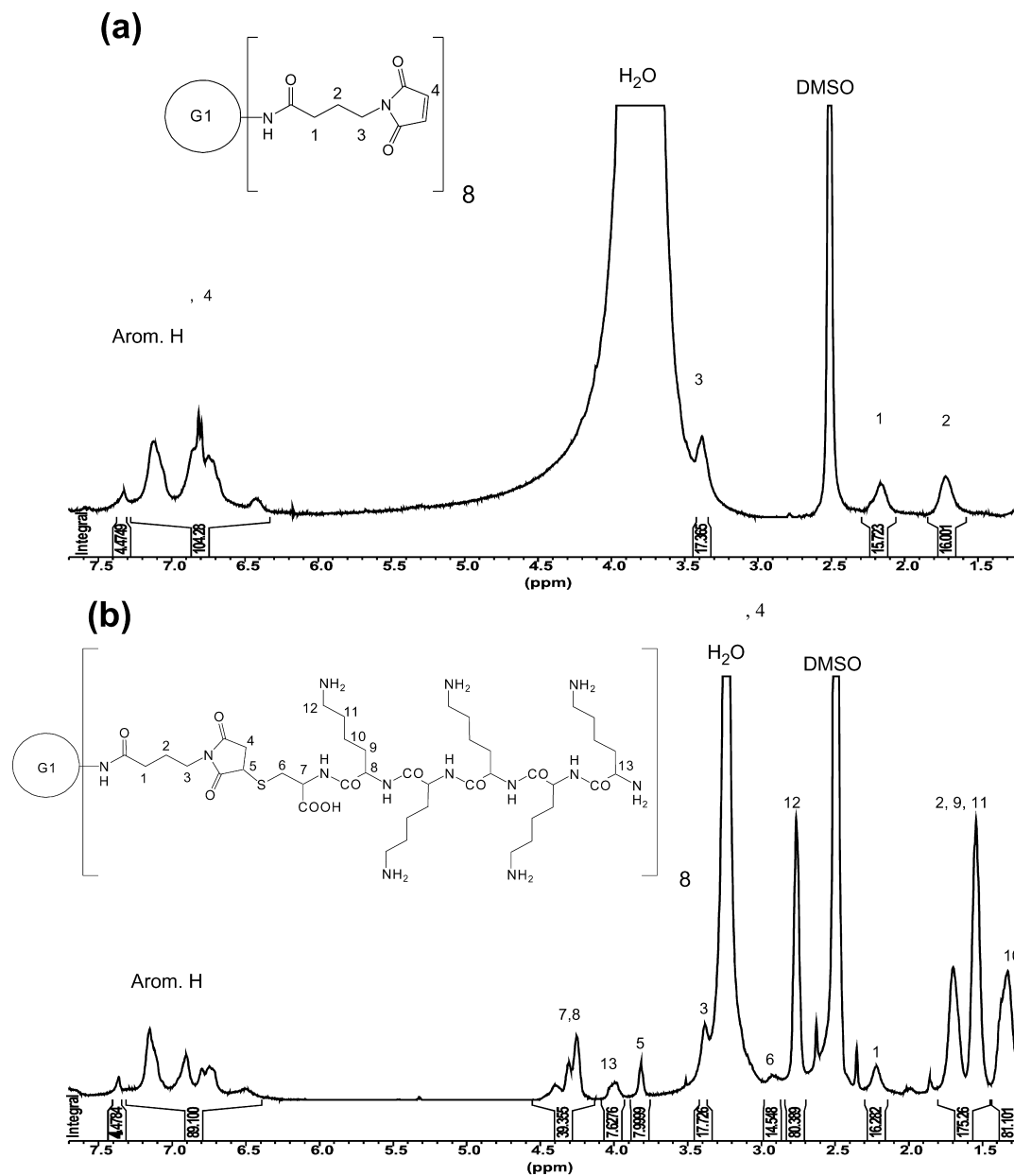
Figure 6. 500 MHz ^1\text{H} NMR-spectra (DMSO- d_6 ) of (a) 8b and (b) 10b .
