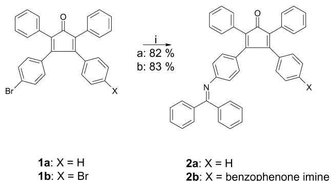
Figure 1. Synthesis of functionalized cyclopentadienones. (i) Benzophenone imine, BINAP, Cs 2 CO 3 , Pd(dba) 2 , toluene.
