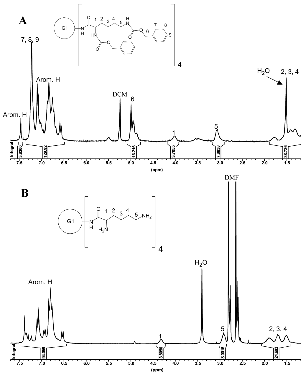
Figure 9. 300 MHz ^1\text{H} NMR-spectra of (a) 18 ( \text{CD}_2\text{Cl}_2 ) and (b) 19 ( \text{DMF } d_6 ).
